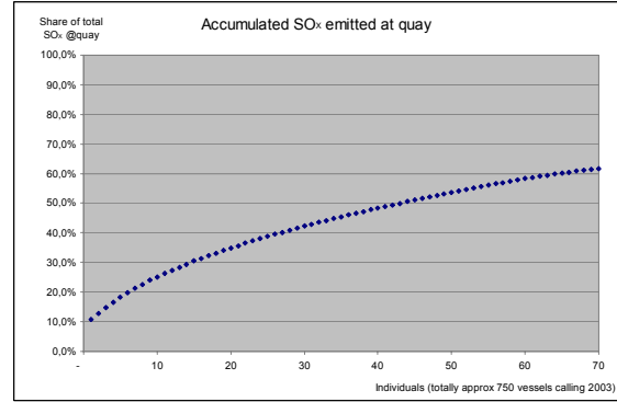
Figure 2 Accumulated emissions of sulphur dioxides emitted at berth for the highest emitting individuals ships. Calculated for vessels calling to the Port of Gothenburg during 2003.
