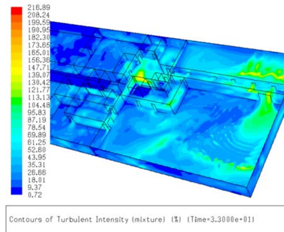
Fig. 20. CFD turbulence intensity after 33 seconds
