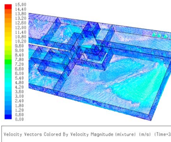
Fig. 19. CFD velocity vectors after 33 seconds
