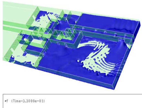
Fig. 18. CFD ISO surfaces after 33 seconds.
