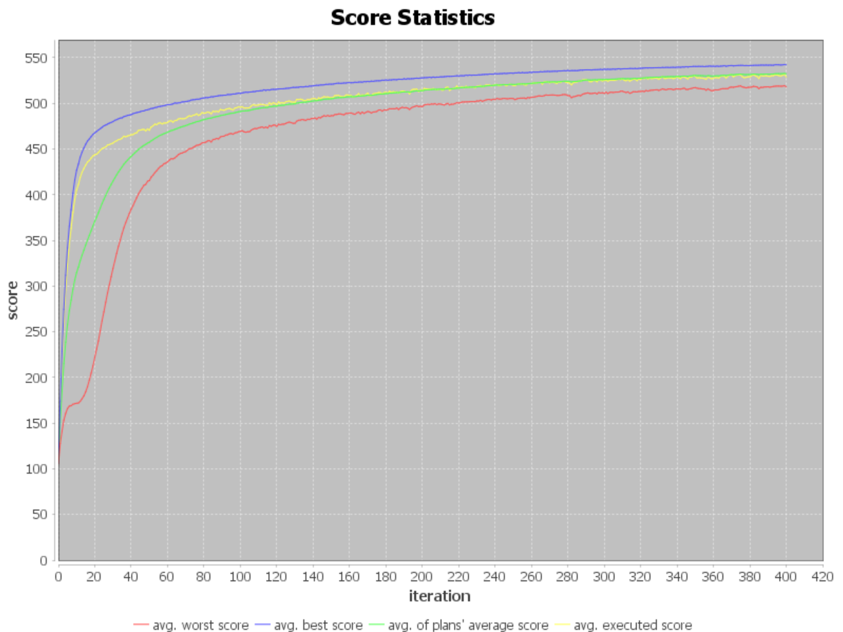
Figure 15: MATSim convergence measures over iterations
